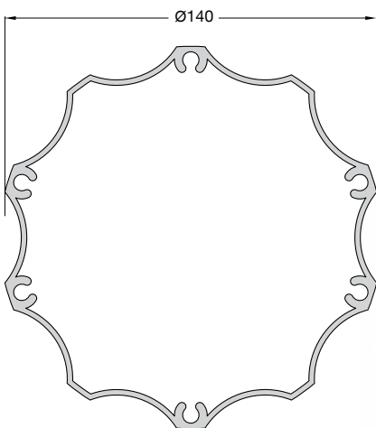
Code: 67 WEIGHT / POIDS: 3153 gr/m COLUMN 140x140 POTEAU 140x140
