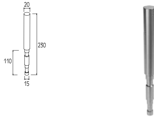
Code: 4188 INFLOOR SUPPORT FOR F50-102 COLUMN FIXATION ENCASTRE DE POTEAU F50-102
