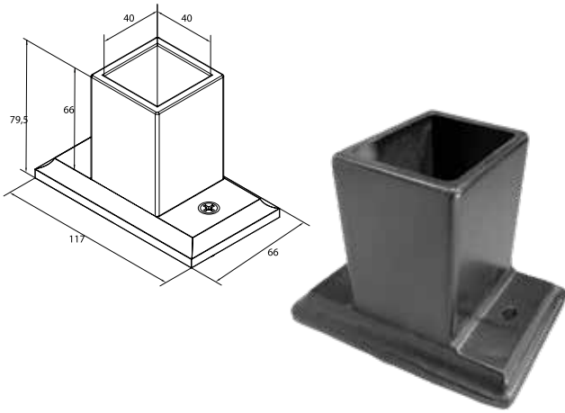
Code: 4113 SUPPORT FOOT FOR COLUMN 40x40 SABOT DE POTEAU 40x40
